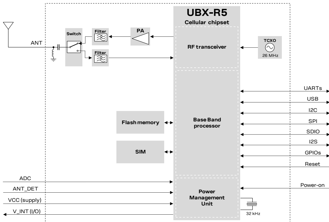
Figure 1: SARA-R500E block diagram
