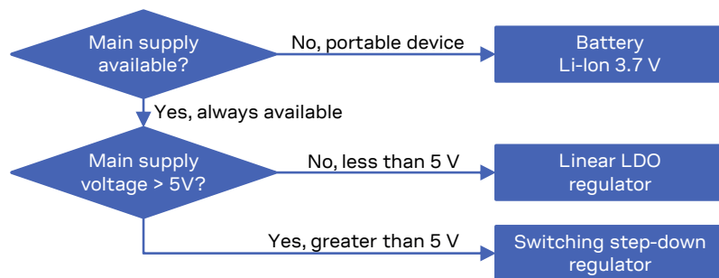
Figure 22: VCC supply concept selection
