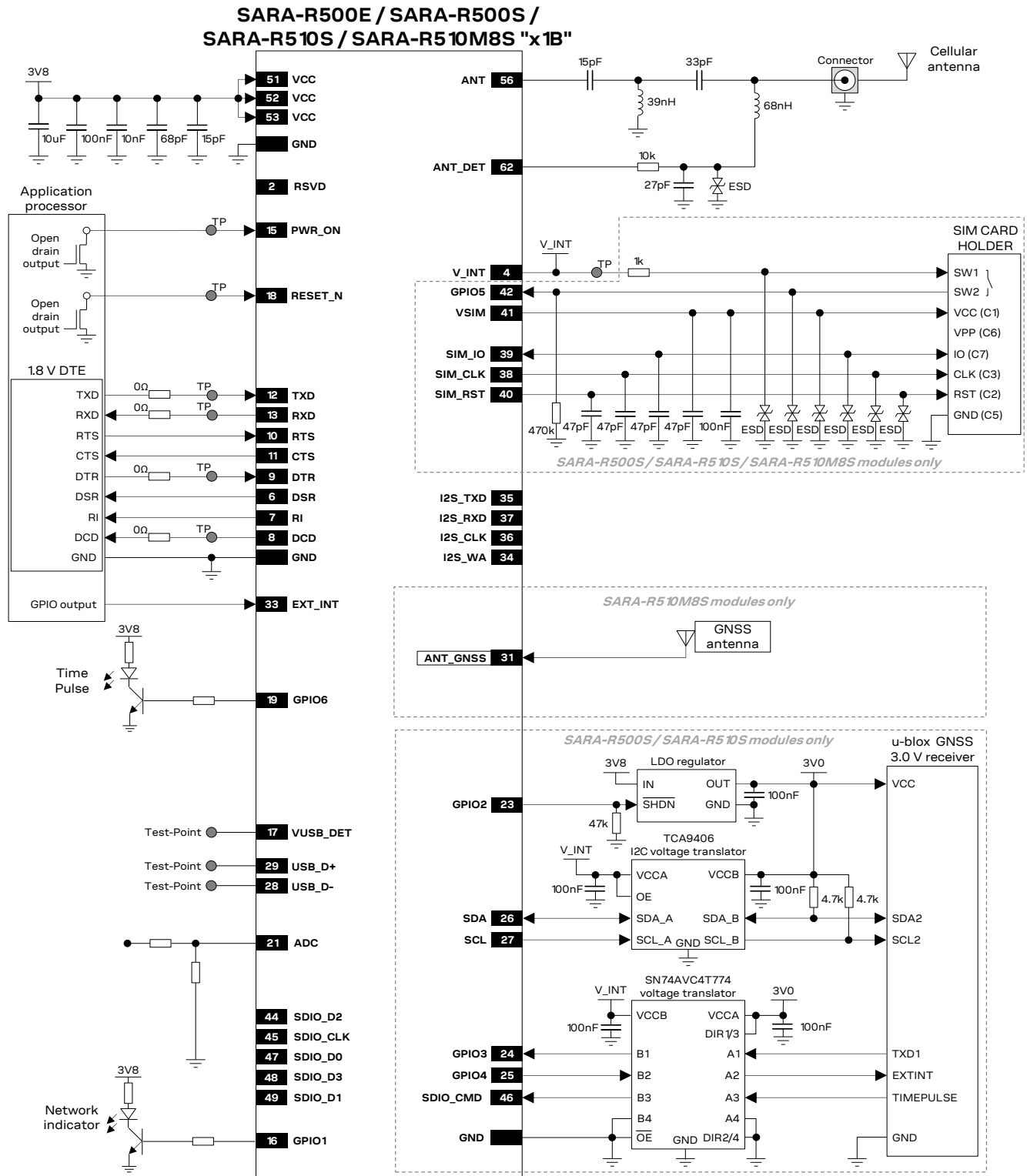
Figure 75: Example schematic diagram integrating a SARA-R500E / SARA-R500S / SARA-R510S / SARA-R510M8S module “x1B” product version
