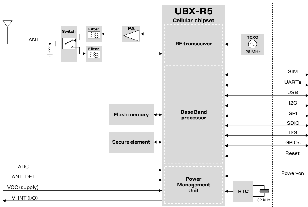
Figure 3: SARA-R510S and SARA-R510AWS block diagram 2
