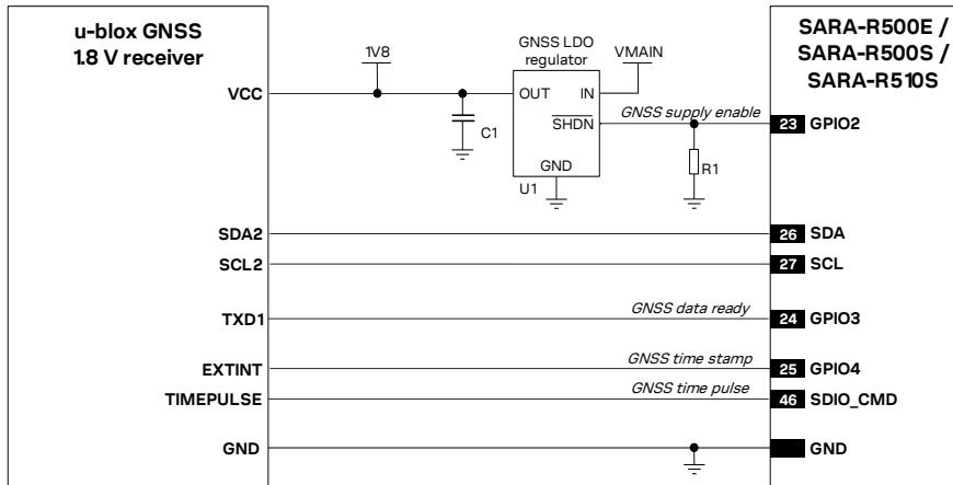
Figure 68: Application circuit for connecting SARA-R500E/R500S/R510S modules to a u-blox 1.8 V GNSS receiver
