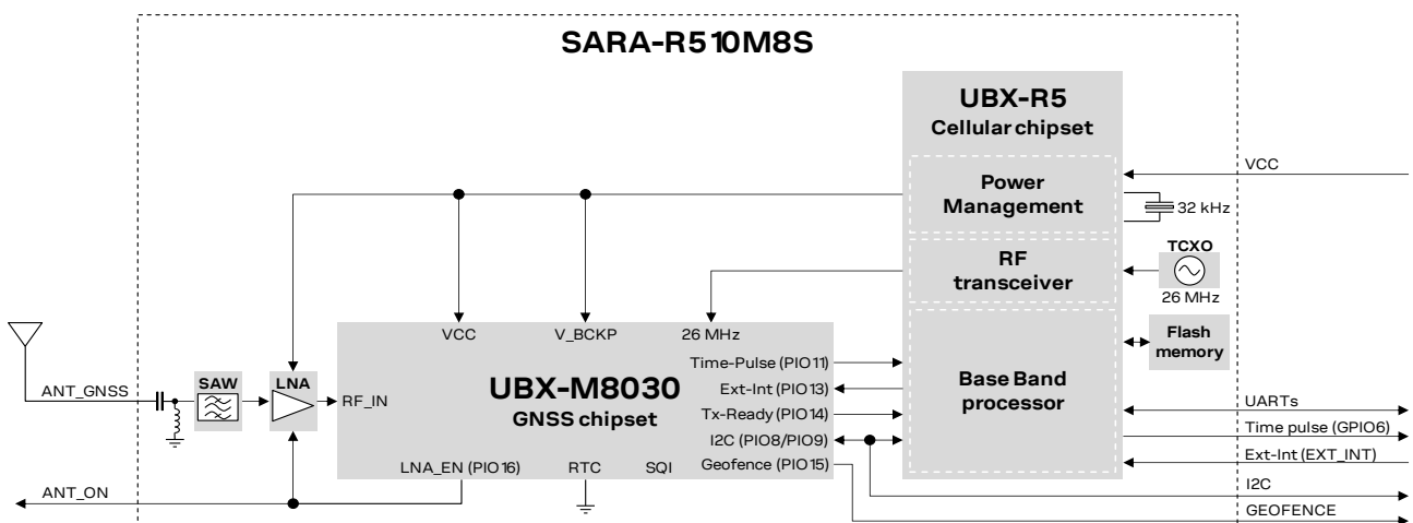
Figure 5: SARA-R510M8S modules GNSS section block diagram
