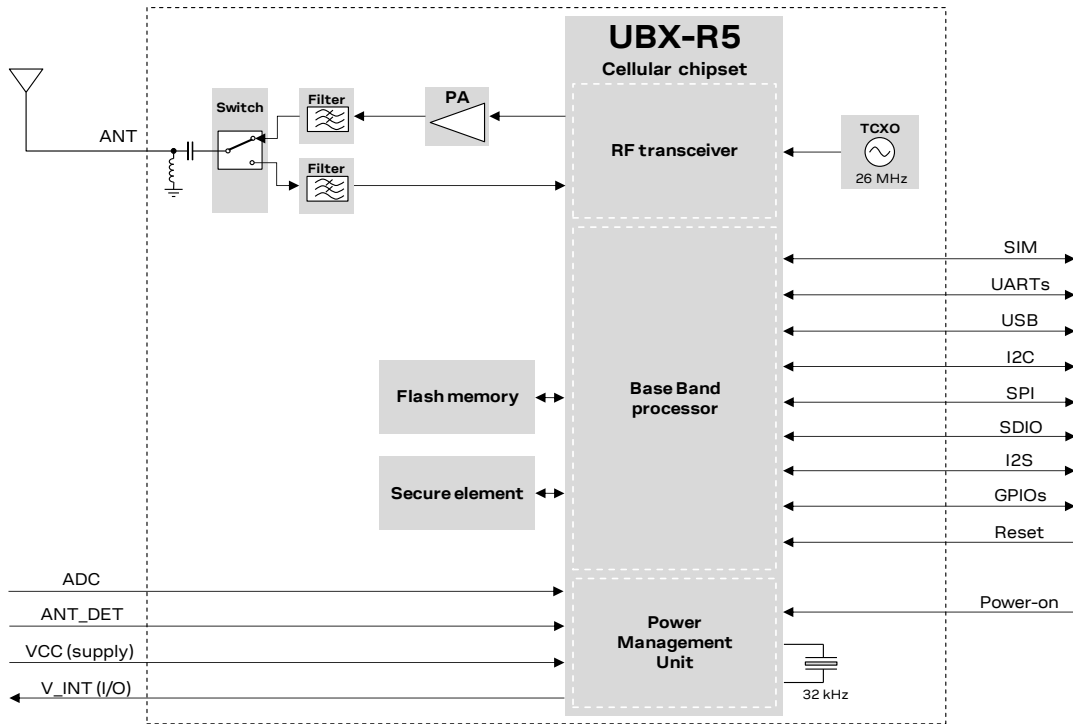
Figure 2: SARA-R500S block diagram 2
