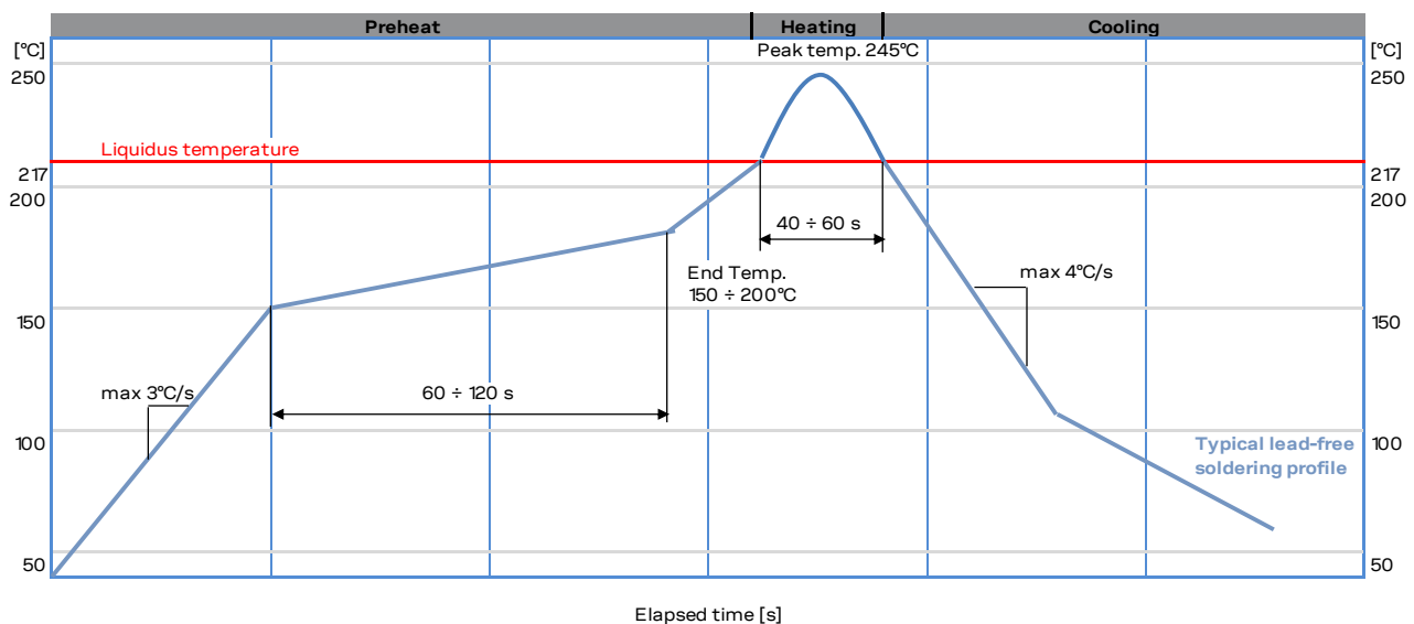
Figure 77: Recommended soldering profile
