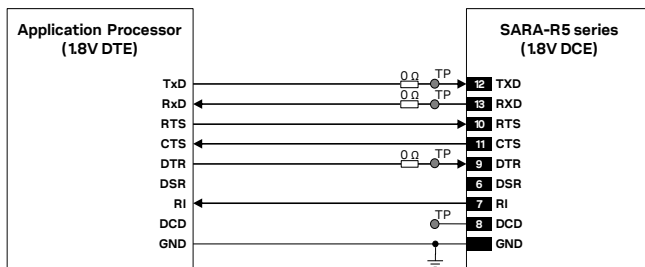
Figure 57: 1 UART interface application circuit with 7-wire link in DTE/DCE serial communication (1.8 V DTE)
