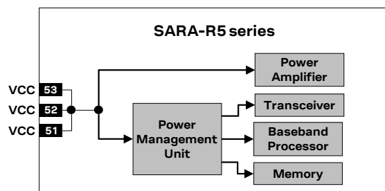
Figure 7: SARA-R5 series modules' internal VCC supply routing
