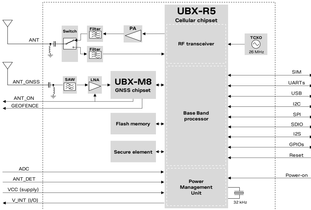
Figure 4: SARA-R510M8S block diagram 2
