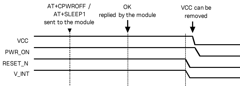
Figure 16: SARA-R5 series modules switch-off sequence by the +CPWROFF/+SLEEP1 AT command
